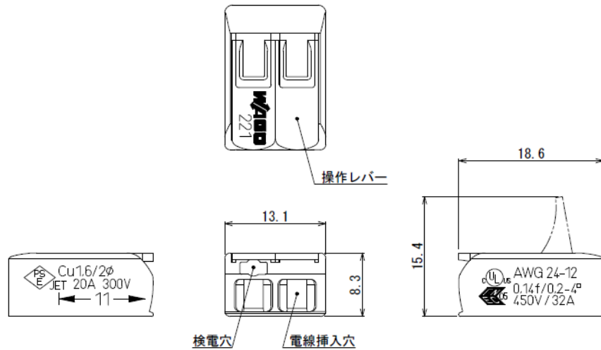
WFR-2-JP, WFR-2BP-JP
