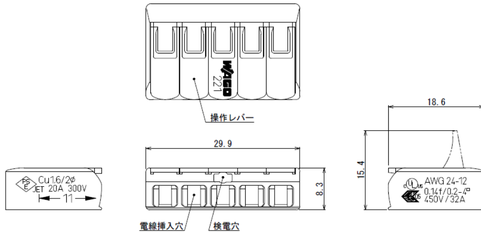
WFR-5-JP, WFR-5BP-JP
