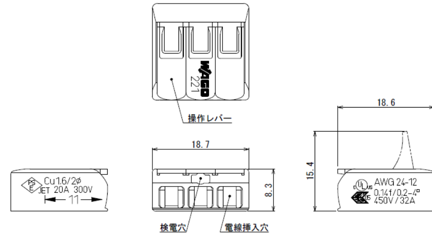
WFR-3-JP, WFR-3BP-JP
