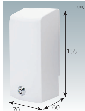
▲RDS21000W-JP
