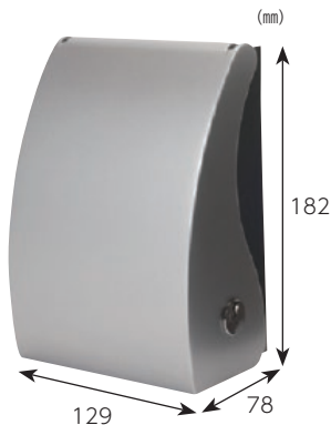
▲RDS10000SL-JP
